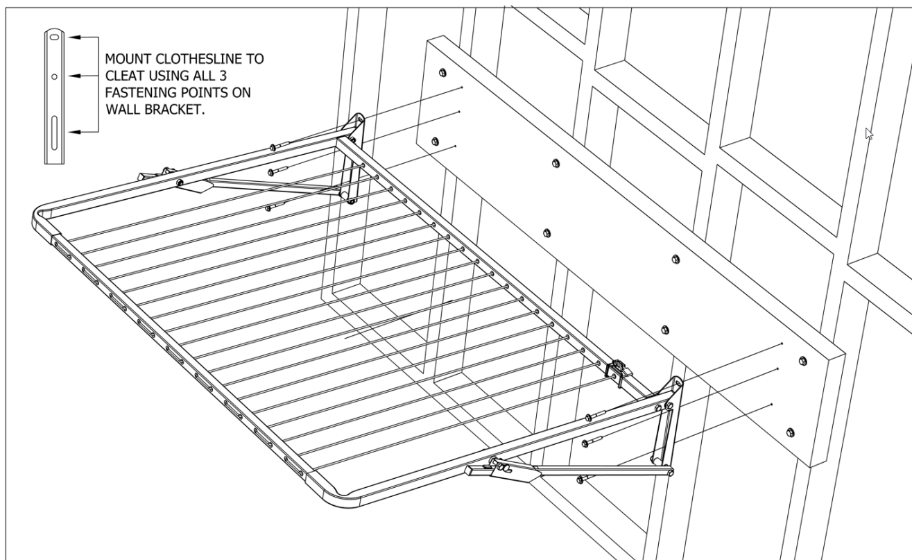
Fig 10. Fitting Balcony Line to cleat.
